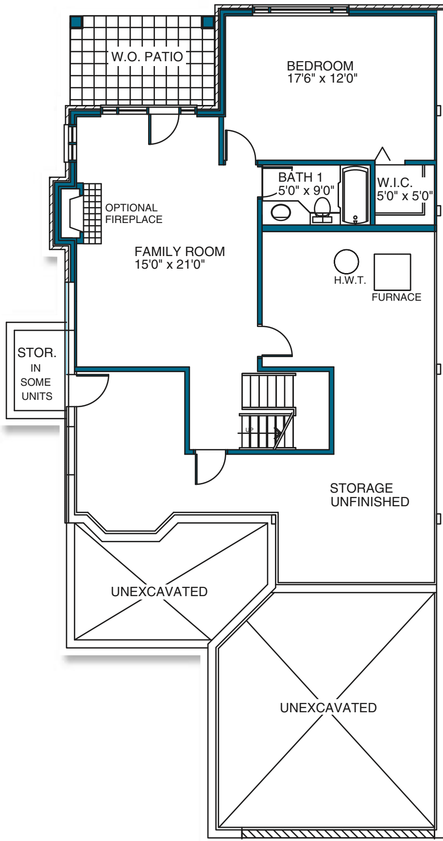
RIVERGLEN GARDEN LEVEL PLAN (OPTIONAL)
