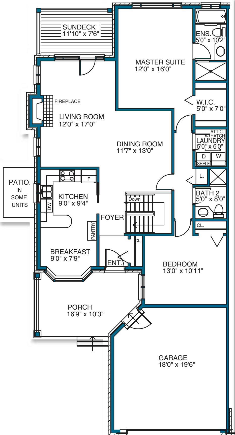
RIVERGLEN MAIN LEVEL PLAN
