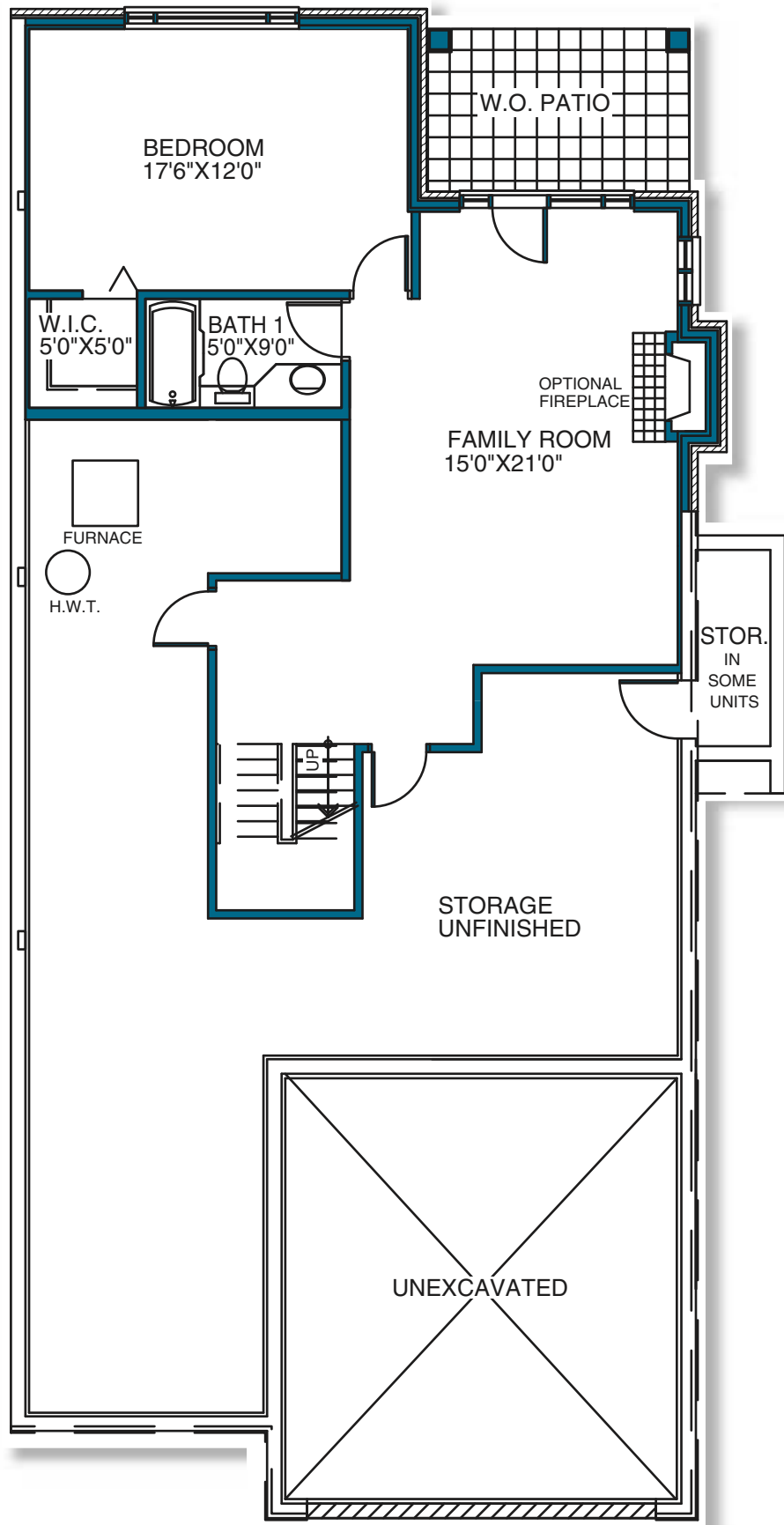
RIVERDALE CLASSIC & RIVERDALE GARDEN LEVEL PLAN (OPTIONAL)
